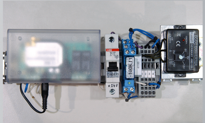
Monitoring refit for ErgoSMS with GSM module
